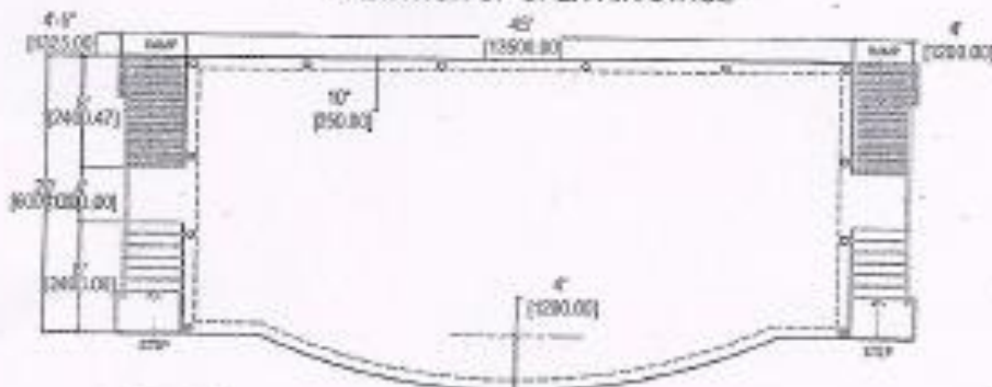
PLAN OF OPEN AIR STAGE
