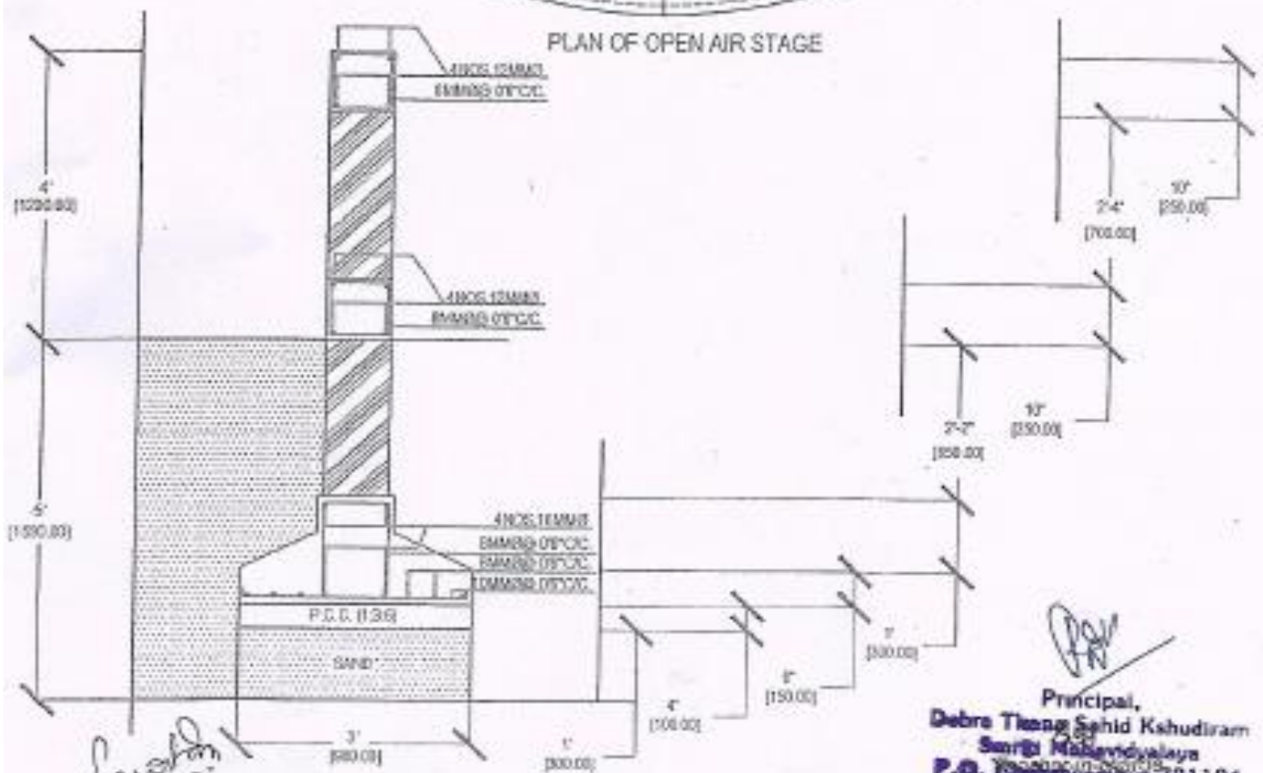
FOUNDATION DETAILS FOR OPEN AIR STAGE
